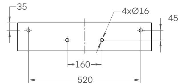
Rear View
