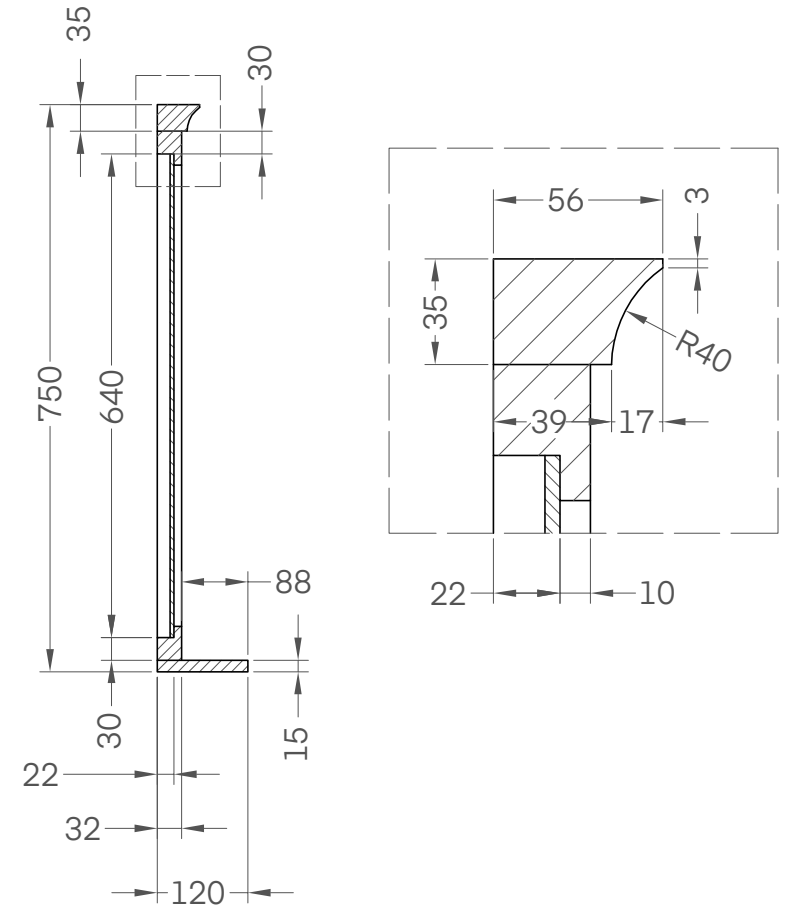
Side View - Section View
