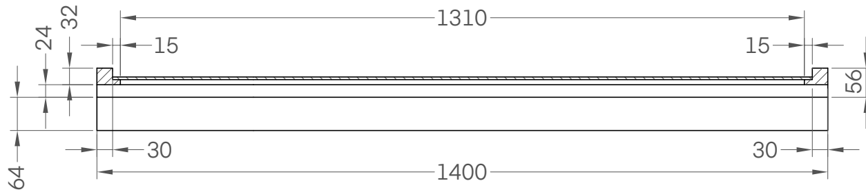
Front View
