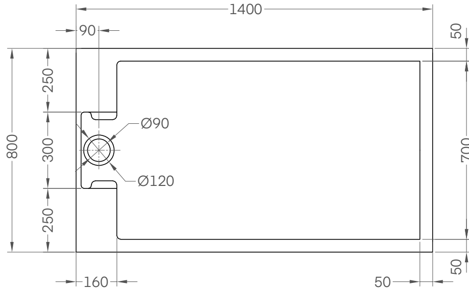
Top View
