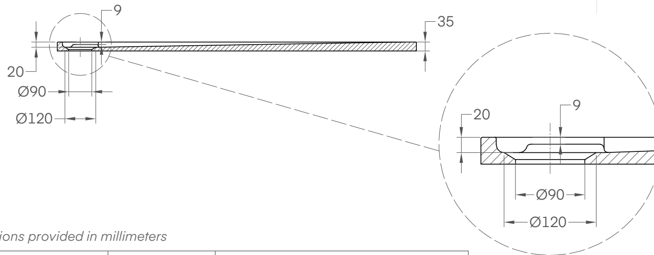
Side View - Section View
