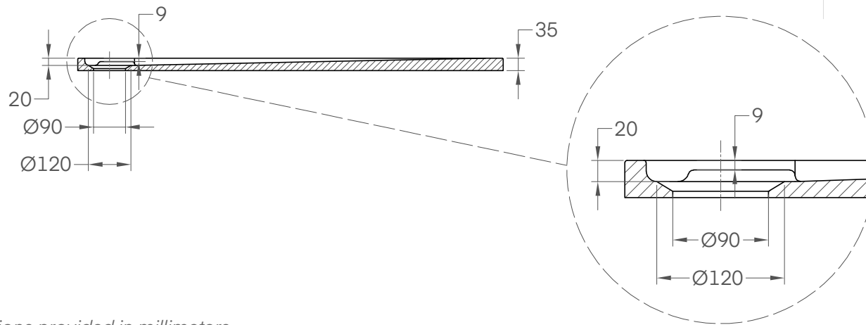
Side View - Section View
