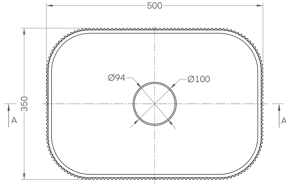
Top View
